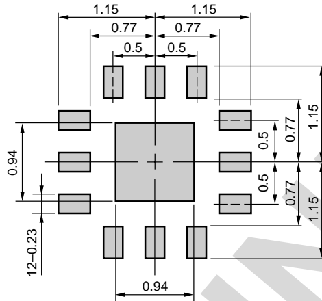
MOUNTING PAD
