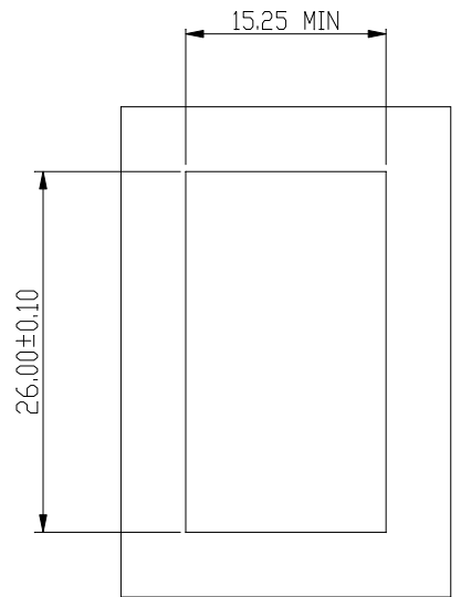
BEZEL CUT-OUT CENTER SPACING DETAIL BEZEL THICKNESS:0.8-2.6
