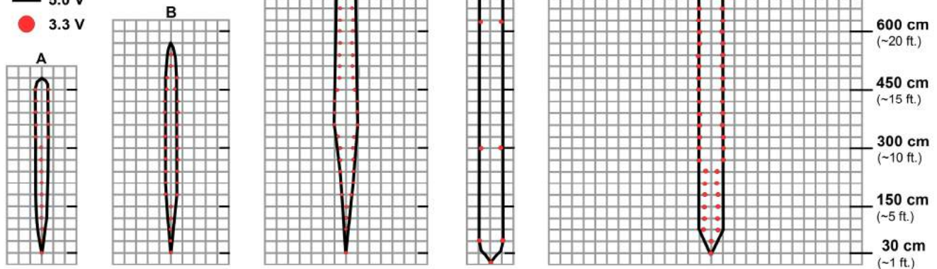
Beam Characteristics are Approximate Beam Pattern drawn to a 1:95 scale for easy comparison to our other products.
