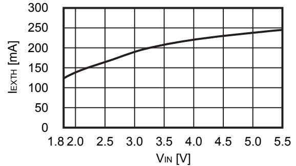
(12) EXT pin output current "L" ( I_{EXTL} ) vs. Input voltage ( V_{IN} )
