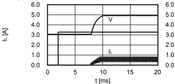
(2) f_{osc} = 1.2\text{ MHz} , I_{OUT} = 600\text{ mA} S-8365AABBA
