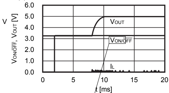
(1) f_{osc} = 1.2\text{ MHz} , I_{OUT} = 1\text{ mA} S-8365AABBA
