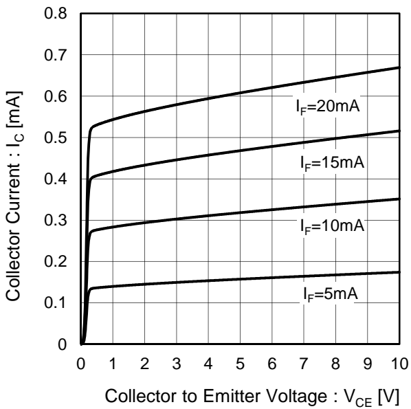
Fig.7 Output Characteristics
