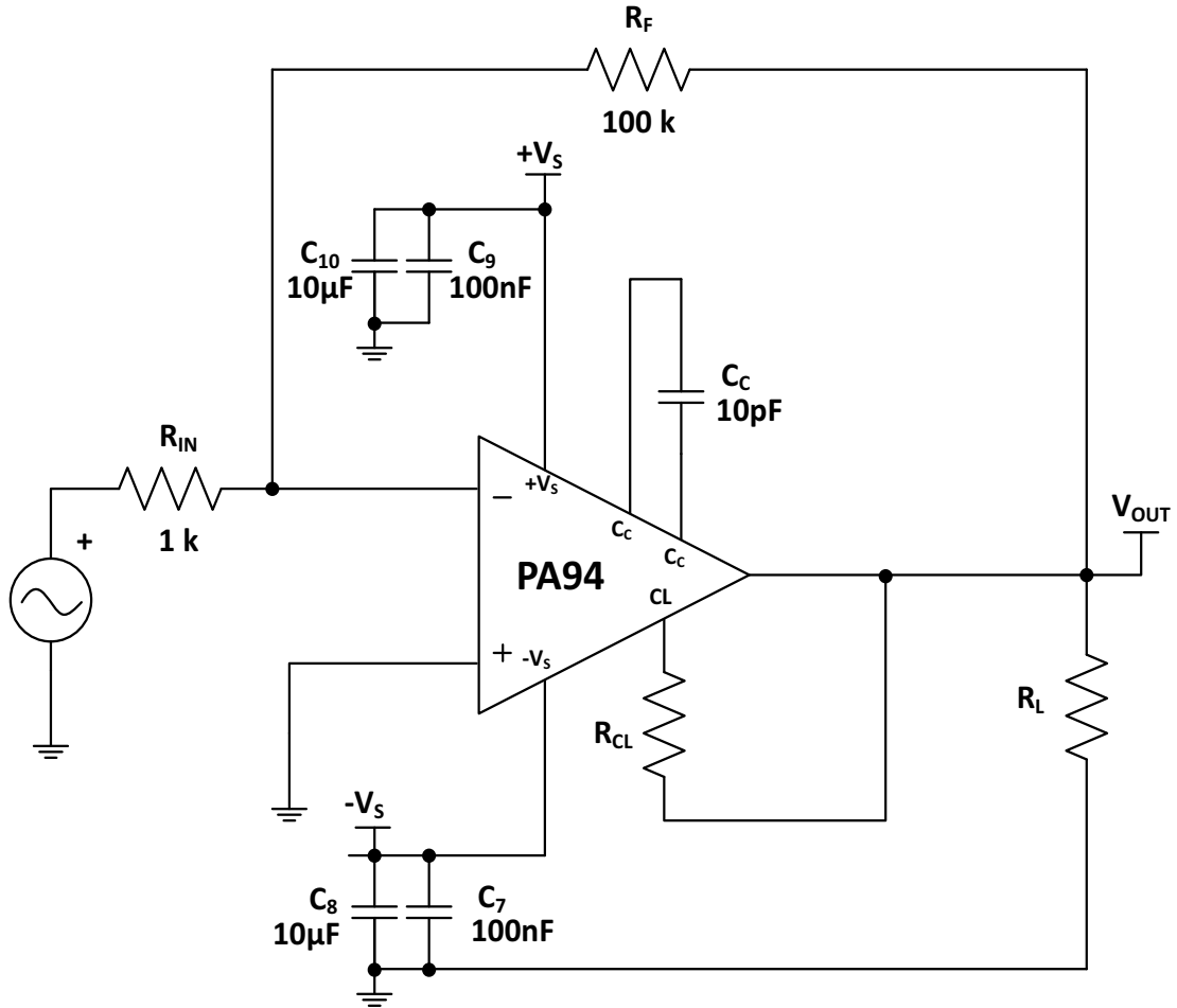
Figure 2: Typical Connection
