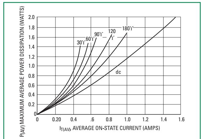
Figure 8. Power Dissipation
