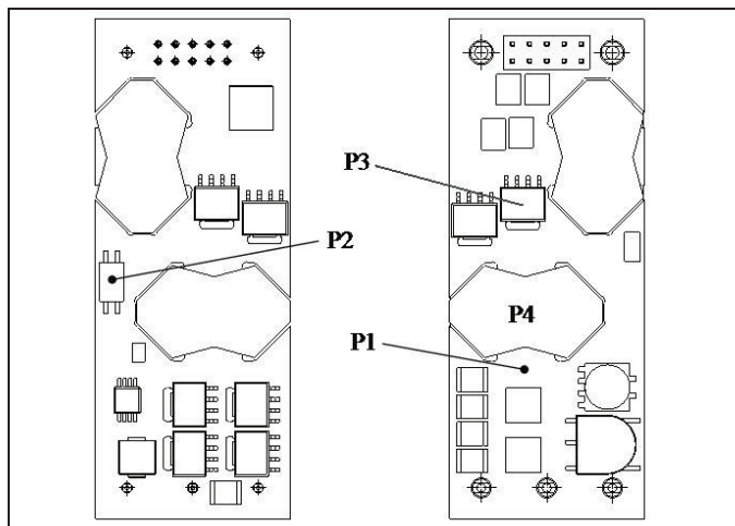
TOP View Open frame Bottom View Open frame and Baseplate
