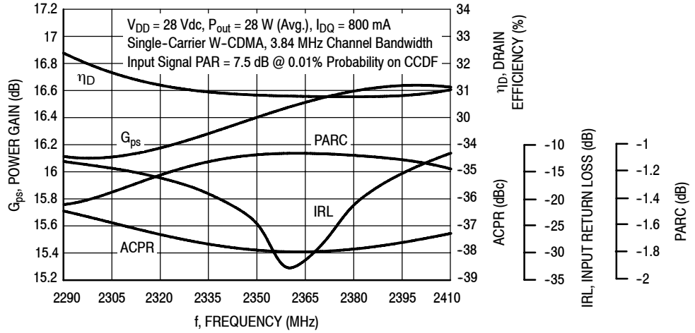
Figure 2. Output Peak-to-Average Ratio Compression (PARC) Broadband Performance @ P_{out} = 28 \text{ Watts Avg.}
