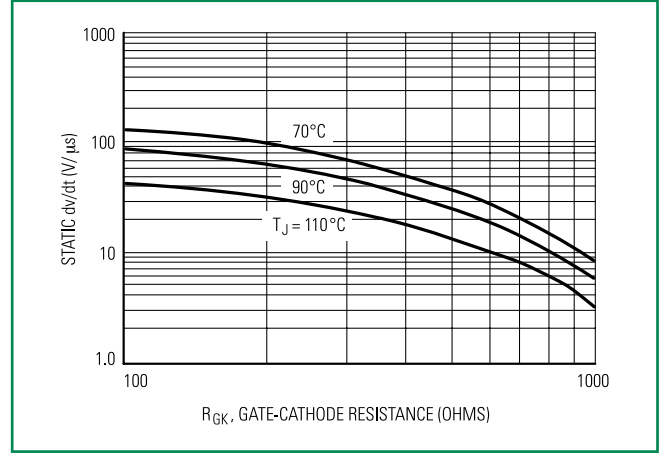
Fig. 10 Exponential Static dv/dt vs Gate-Cathode Resistance & Junction Temp
