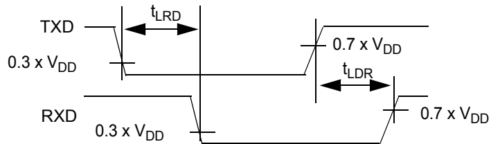
Figure 11. CAN Signal Propagation Loop Delay TXD to RXD
