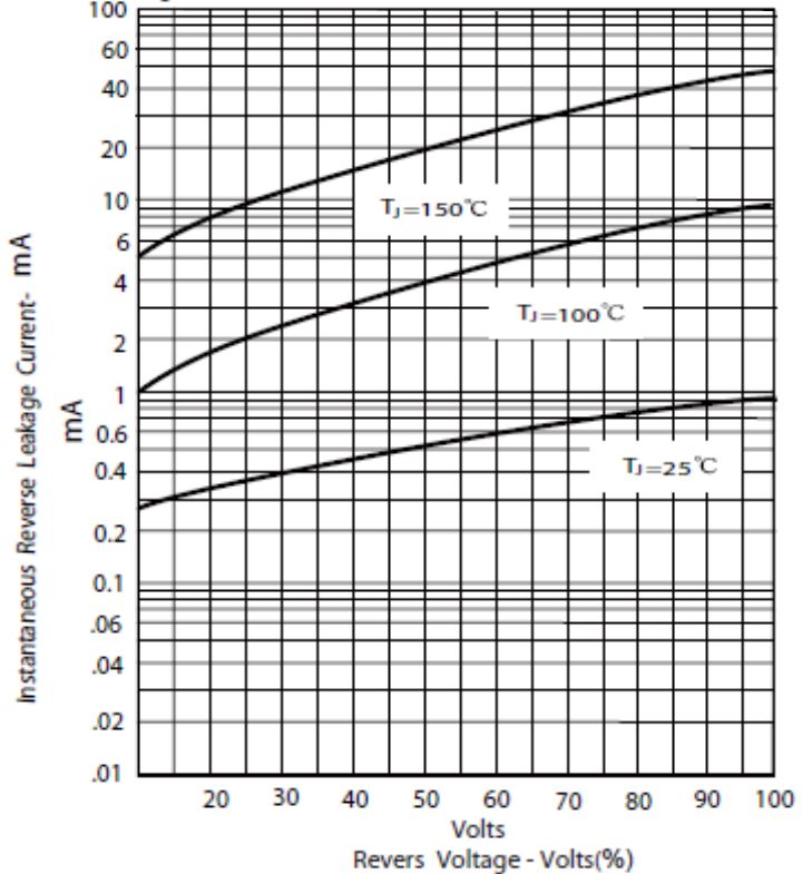
Figure.4-Typical Reverse Characteristics
