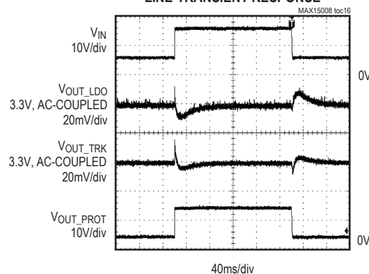
LINE-TRANSIENT RESPONSE
