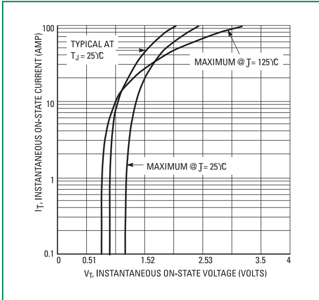
Figure 7. On-State Characteristics
