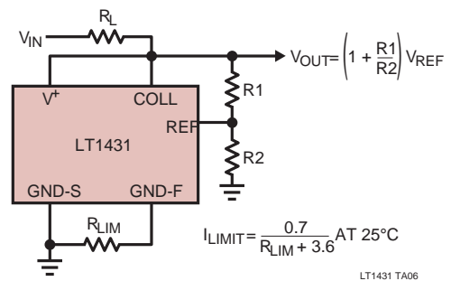
Programmable Reference with Adjustable Current Limit
