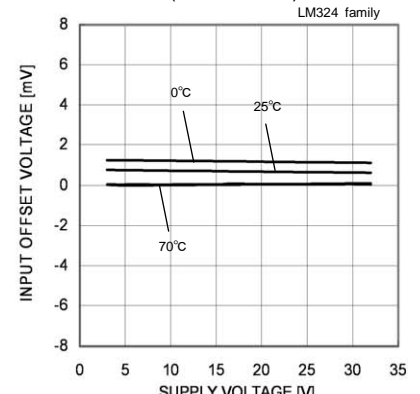
Input Offset Voltage - Supply Voltage (Vicm=0[V], VOUT=1.4[V])
