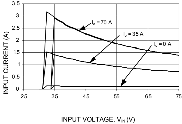
Figure 37. Typical Start-Up (Input Current) characteristics at room temperature.
