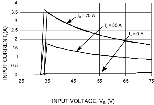
Figure 31. Typical Start-Up (Input Current) characteristics at room temperature.
