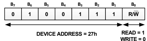
FIGURE 19. DEVICE ADDRESS BYTE FORMAT
