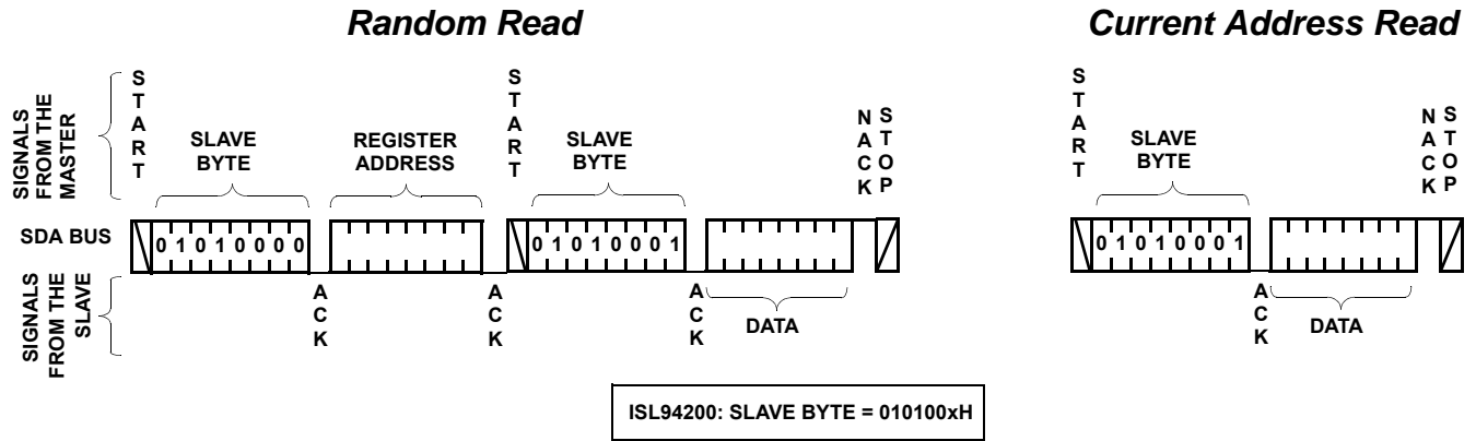
FIGURE 12. READ SEQUENCE
