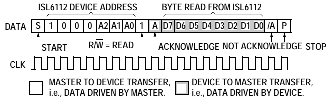
FIGURE 35. RECEIVE_BYTE PROTOCOL
