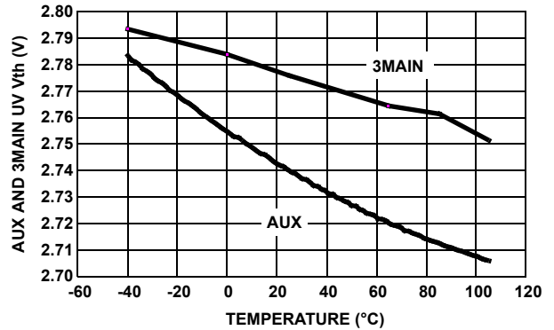
FIGURE 12. AUX AND 3.3MAIN POWER GOOD THRESHOLD VOLTAGE vs TEMPERATURE
