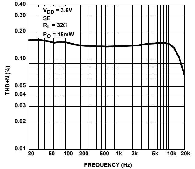
FIGURE 6. THD+N vs FREQUENCY
