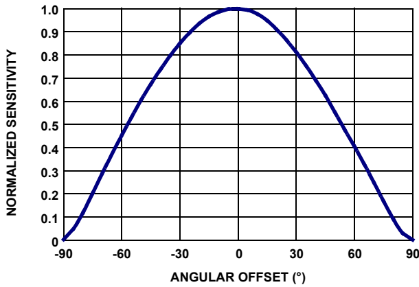
FIGURE 8. ANGULAR SENSITIVITY
