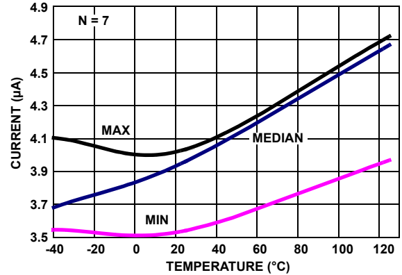
FIGURE 26. ISL28276 SUPPLY CURRENT vs TEMPERATURE, V_+, V_- = \pm 2.5V DISABLED, R_L = INF
