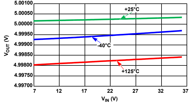
FIGURE 39. LINE REGULATION, THREE TEMPERATURES
