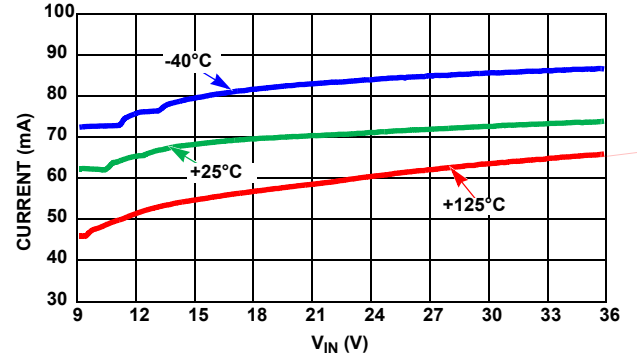
FIGURE 65. SHORT-CIRCUIT TO V IN
