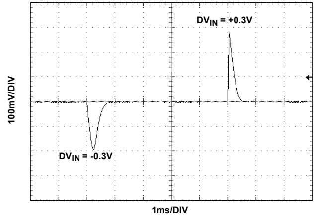
FIGURE 6. LINE TRANSIENT RESPONSE, C_L = 0nF
