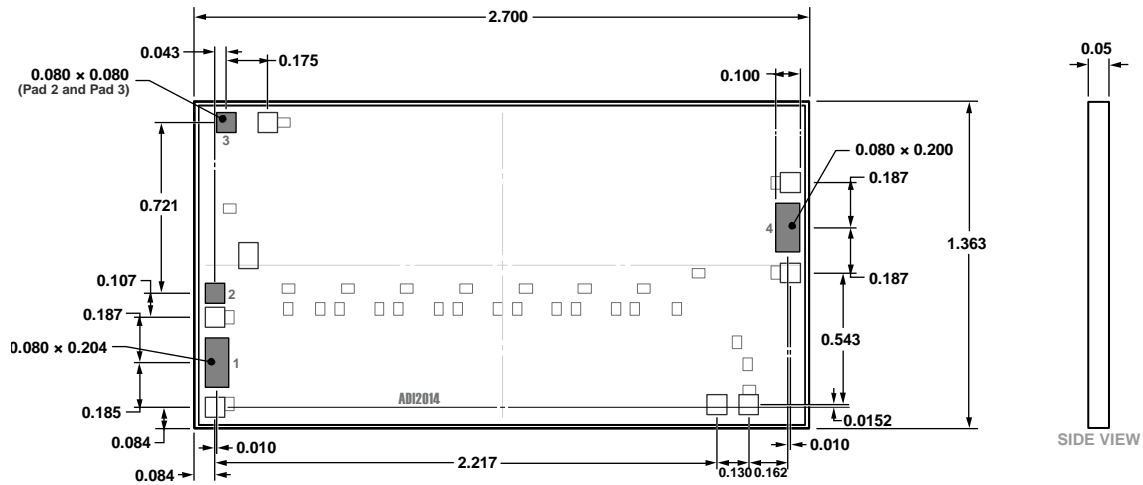
Figure 41. 4-Pad Bare Die [CHIP] (C-4-3) Dimensions shown in millimeter
