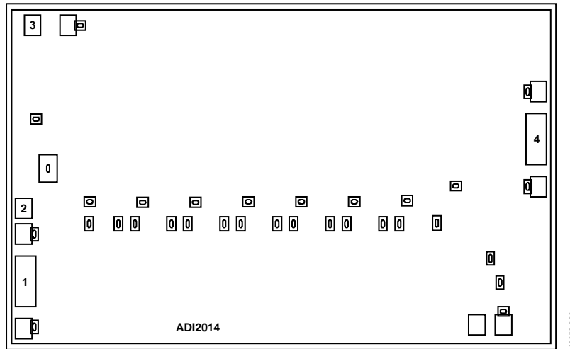
Figure 2. Pad Configuration
