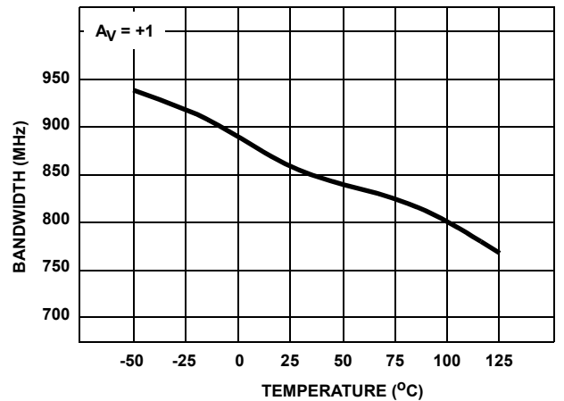
FIGURE 10. -3dB BANDWIDTH vs TEMPERATURE
