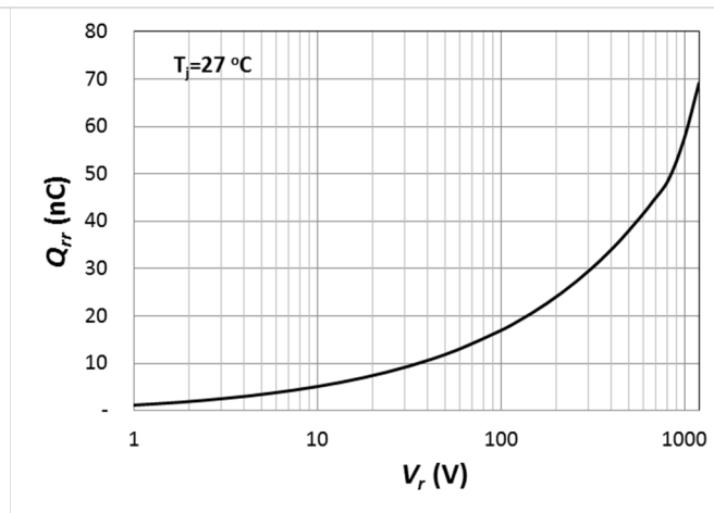
Fig. 22 Recovery Charge
