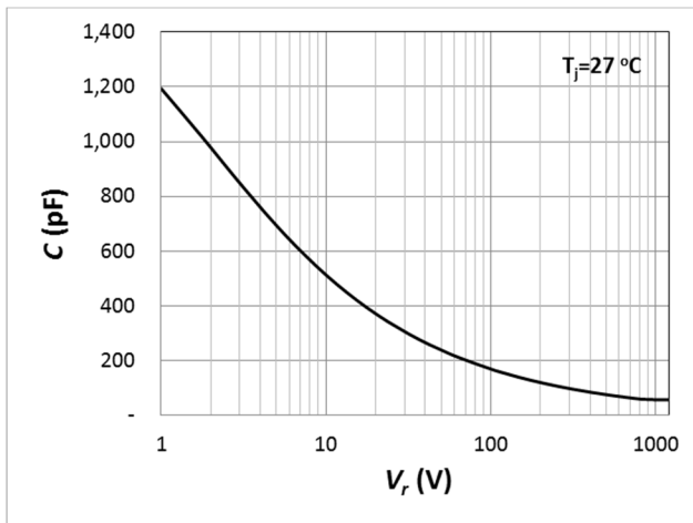
Fig. 21 Capacitance Curve
