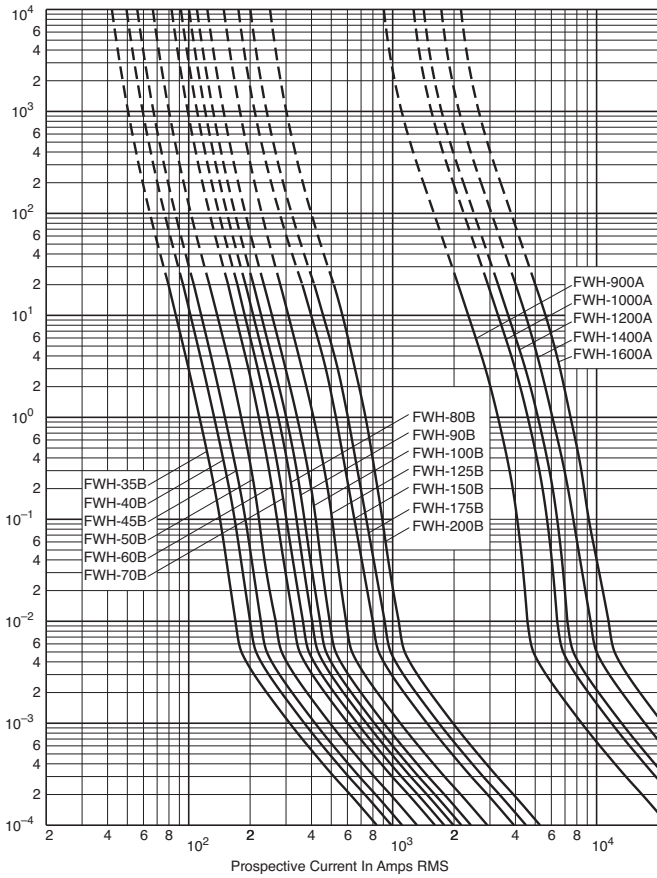
Time-Current Curve
