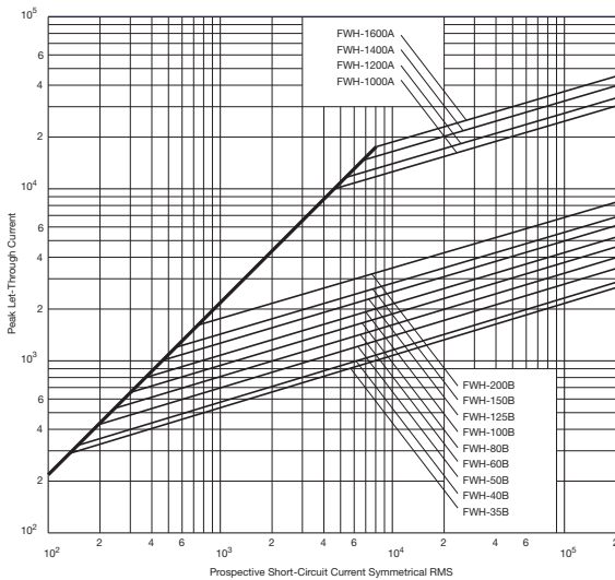
Peak Let-Through Curve
