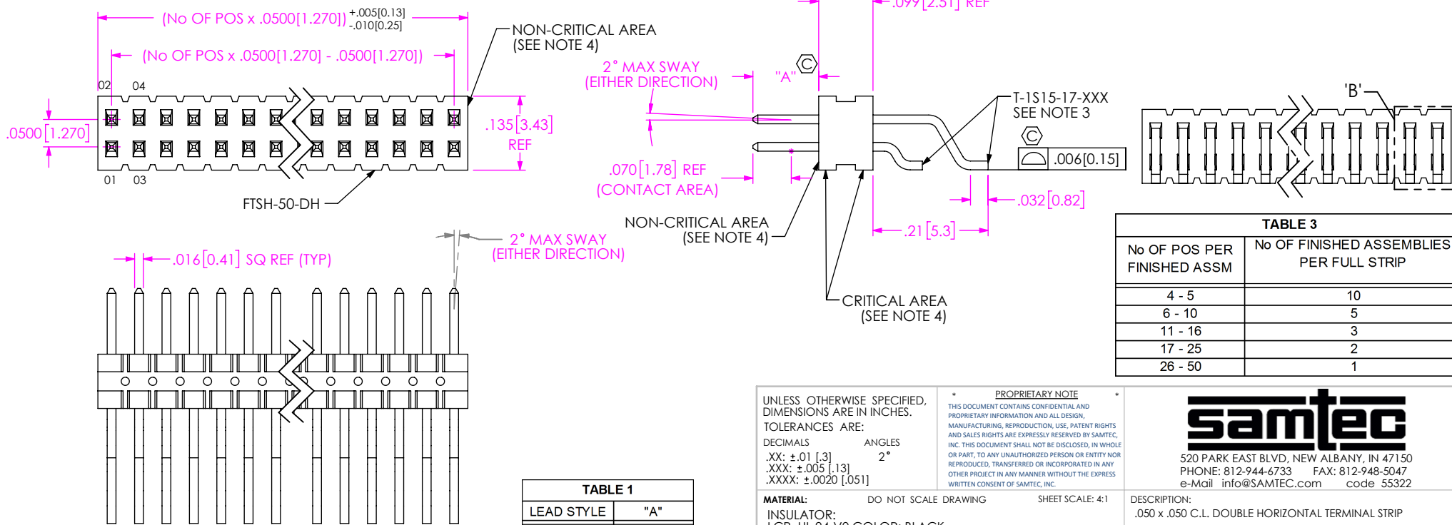
FIG 1 FTSH-1XX-XX-XXX-DH SHOWN
