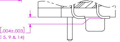
DETAIL 'K' TOP ROW TAIL (LOCATE ASSY ON DATUM -C- FOR MEASUREMENT)
