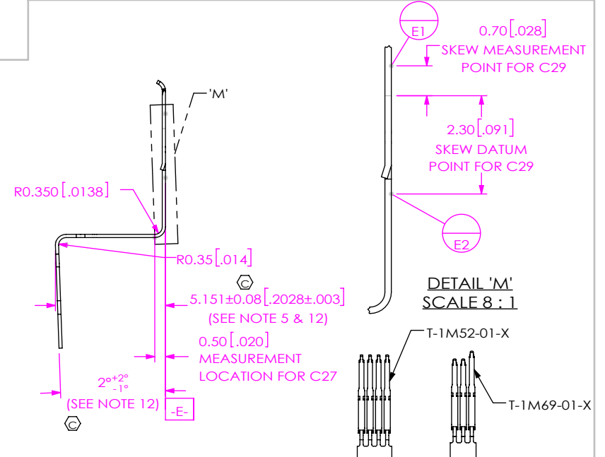
IN-PROCESS 7 (FORM 2 TERMINAL T-1M52-01-X & T-1M69-01-X)
