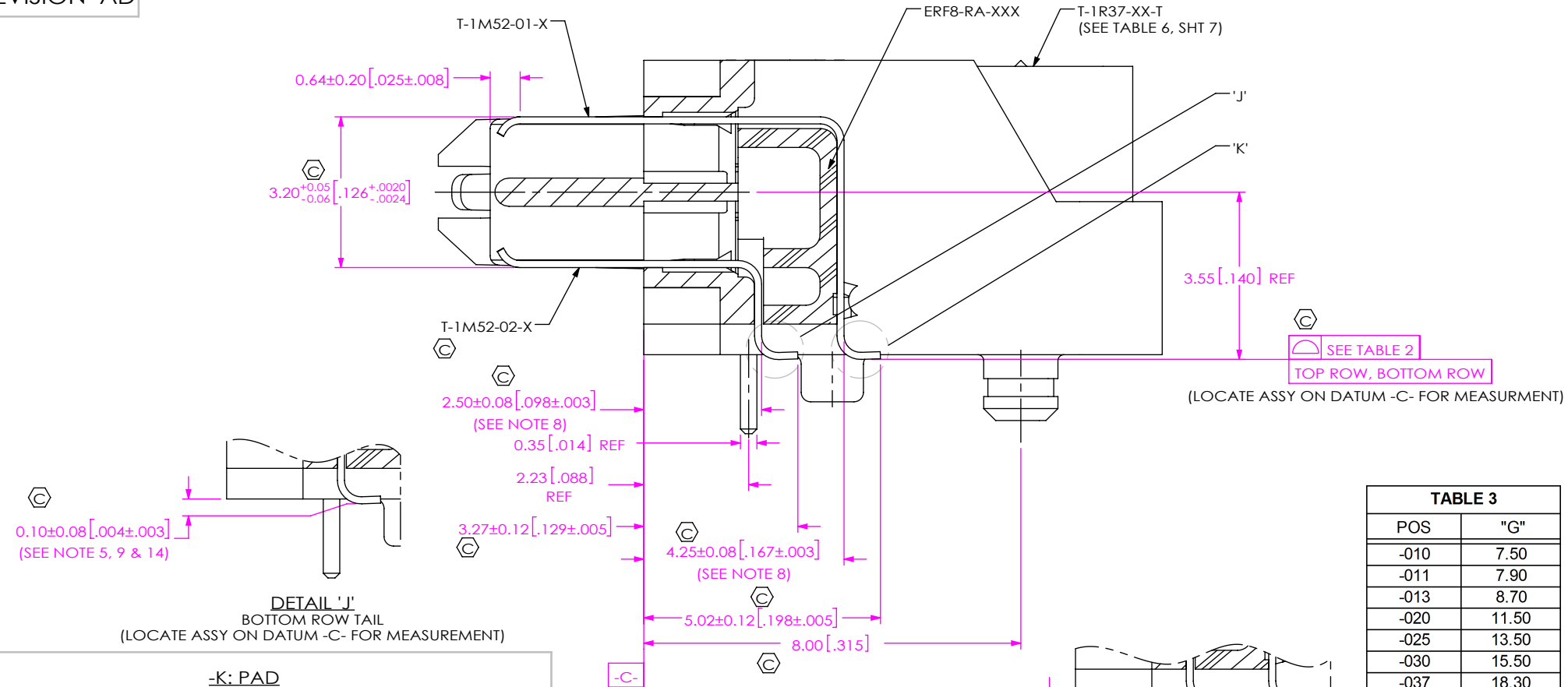
-K: PAD ERM8-030-01-X-D-RA-L-K SHOWN (USE K-DOT-.236-.343-.005)
