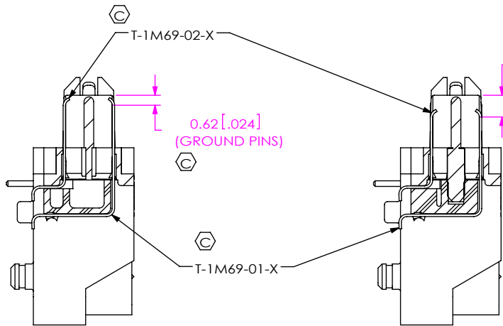
SECTION "B"-"B" SCALE 3 : 1
