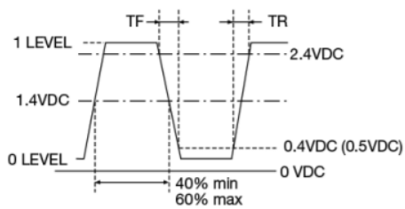
Figure 2) TTL Output Wave Form
