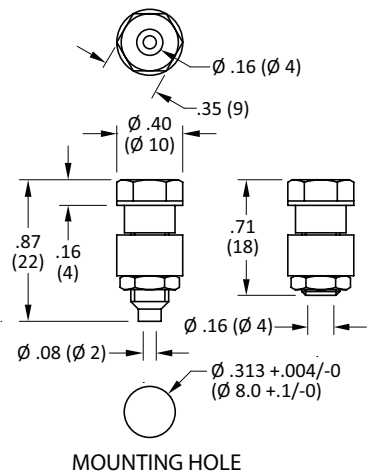
MOUNTING HOLE
