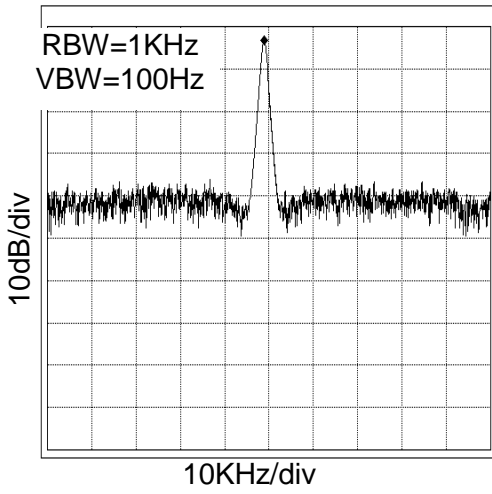
Figure 9. 108MHz Spectrum (At V_{DD}=3.3V and C_L=15pF )
