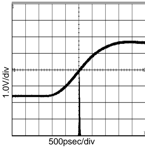
Figure 11. 98MHz Period-Jitter (At V_{DD}=3.3V and C_L=15pF )
