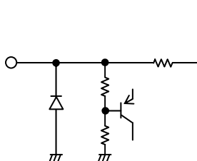
9pin<TEST>
