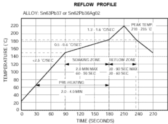
Figure 37. Reflow Profile.
