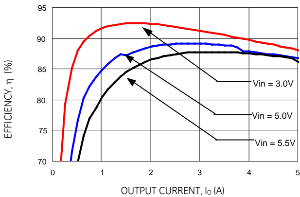
Figure 3. Converter Efficiency versus Output Current (Vout = 1.5Vdc).
