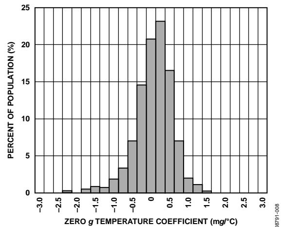
Figure 8. Z-Axis Zero-g Bias Drift, V_S = V_{DD/IO} = 3.3 V
