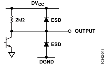
Figure 28. Logic Output
