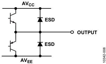
Figure 25. Analog Output
