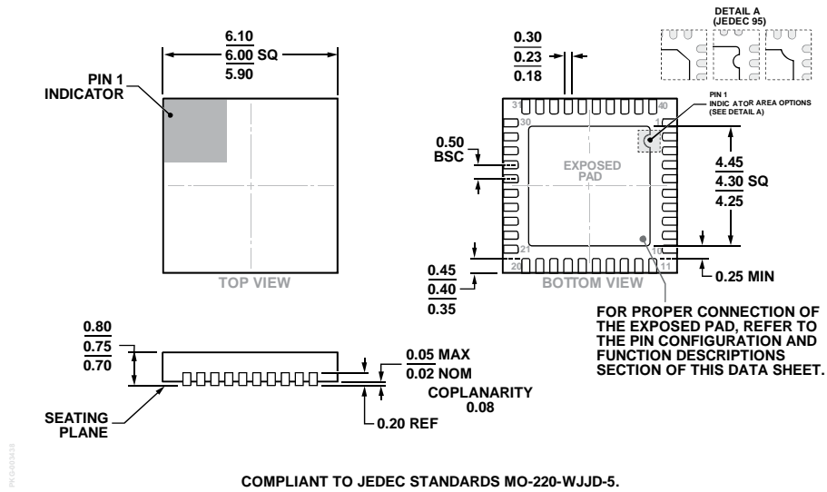
COMPLIANT TO JEDEC STANDARDS MO-220-WJJD-5. Figure 29. 40-Lead Lead Frame Chip Scale Package [LFCSP] 6 mm × 6 mm Body and 0.75 mm Package Height (CP-40-10) Dimensions shown in millimeters
