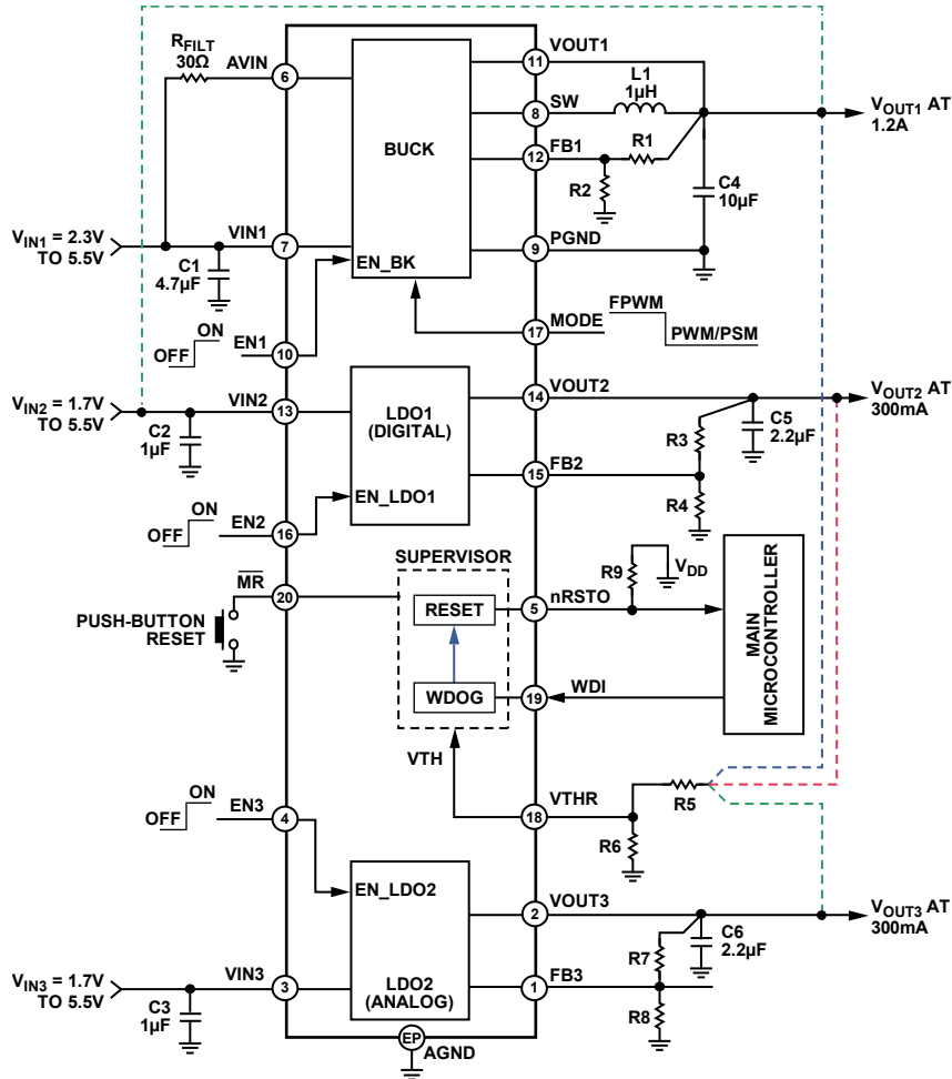
Figure 113. Application Diagram
