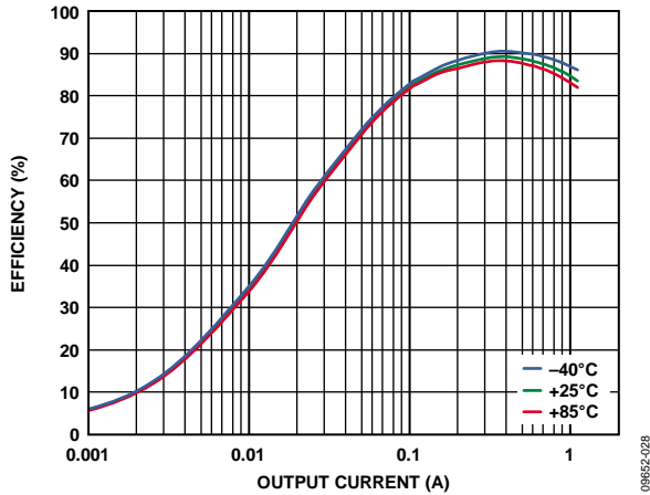
Figure 28. Buck Efficiency vs. Load Current, Across Temperature, V_{IN} = 5.0V , V_{OUT1} = 1.8V , PWM Mode
