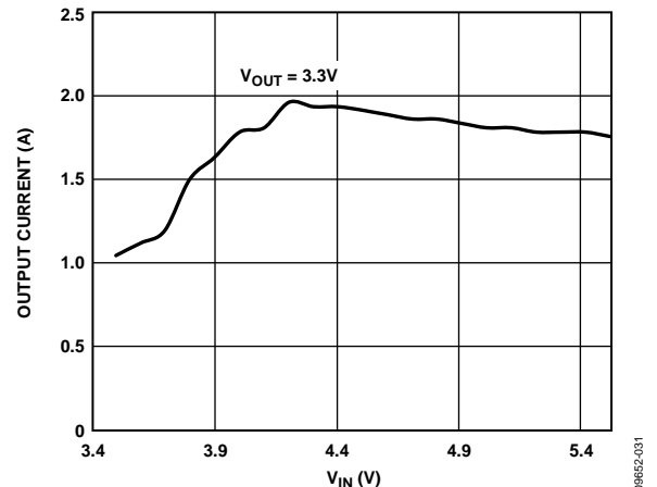
Figure 31. Buck DC Current Capability vs. Input Voltage
