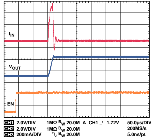
Figure 60. LDO1, LDO2 Startup, V_{OUT} = 3.3\text{ V} , I_{OUT} = 5\text{ mA}
