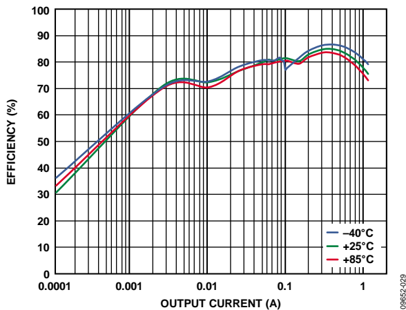
Figure 29. Buck Efficiency vs. Load Current, Across Temperature, V_{IN} = 5.0V , V_{OUT1} = 1.2V , Auto Mode
