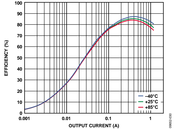
Figure 30. Buck Efficiency vs. Load Current, Across Temperature, V_{IN} = 5.0V , V_{OUT1} = 1.2V , PWM Mode
