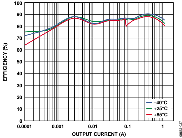
Figure 27. Buck Efficiency vs. Load Current, Across Temperature, V_{IN} = 5.0V , V_{OUT1} = 1.8V , Auto Mode
