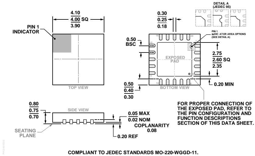
Figure 110. 20-Lead Lead Frame Chip Scale Package [LFCSP] 4 mm × 4 mm Body and 0.75 mm Package Height (CP-20-8) Dimensions shown in millimeters
