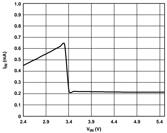
Figure 5. System Quiescent Current (Sum of All the Input Currents) vs. Input Voltage, VOUT1 = 1.8 V, VOUT2 = VOUT3 = 3.3 V (UVLO = 3.3 V)
