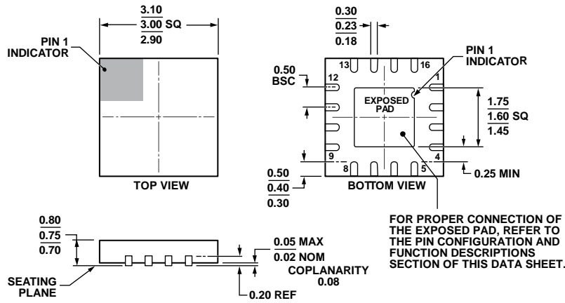
Figure 47. 16-Lead Lead Frame Chip Scale Package [LFCSPP] 3 mm x 3 mm Body and 0.75 mm Package Height (CP-16-22) Dimensions shown in millimeters
