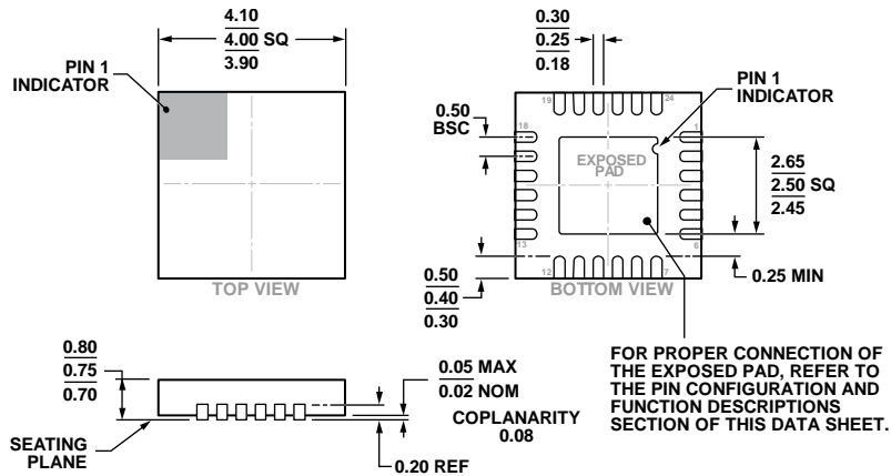
Figure 76. 24-Lead Lead Frame Chip Scale Package [LFCSP_WQ] 4 mm × 4 mm Body, Very Very Thin Quad (CP-24-7) Dimensions shown in millimeters
