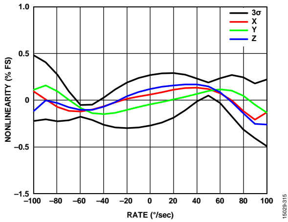
Figure 13. Gyroscope Nonlinearity
