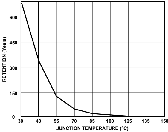
Figure 45. Flash Memory Retention
