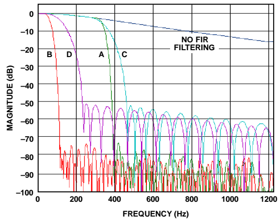
Figure 47. FIR Filter Frequency Response Curves
