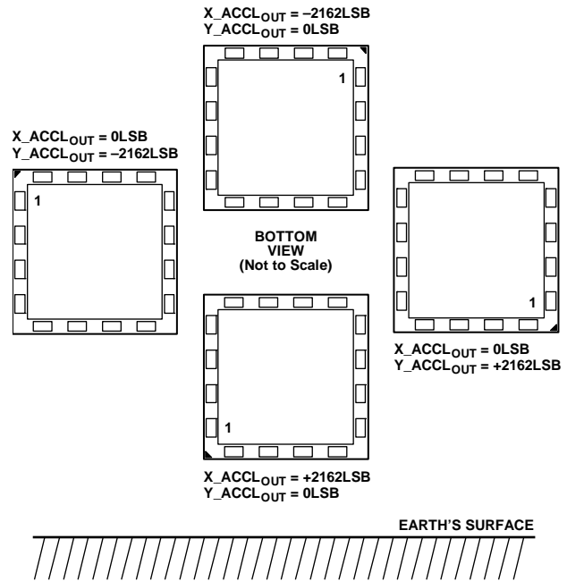
Figure 36. Output Response vs. Orientation
