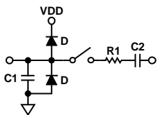
Figure 35. Equivalent Analog Input Circuit Conversion Phase: Switch Open Track Phase: Switch Closed
