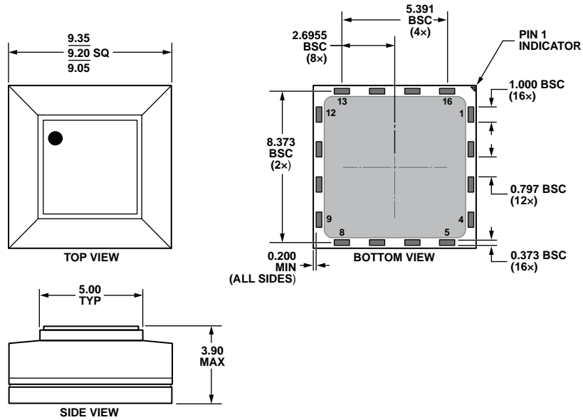
Figure 38. 16-Terminal Stacked Land Grid Array [LGA] (CC-16-2) Dimensions shown in millimeters
