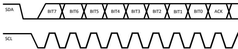
Figure 13. Serial Interface Protocol
