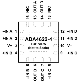
Figure 7. 16-Lead LFCSP Pin Configuration, ADA4622-4
