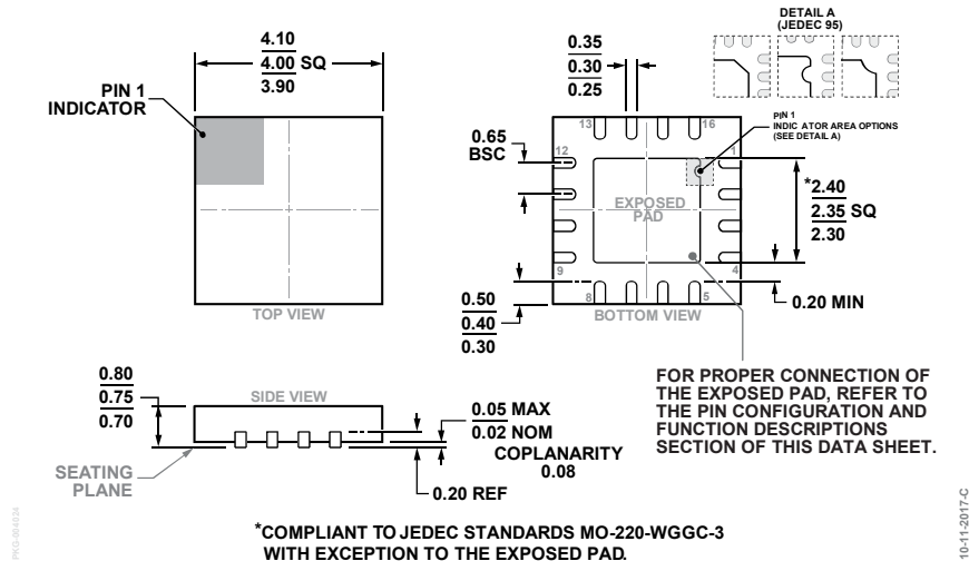
Figure 108. 16-Lead Lead Frame Chip Scale Package [LF CSP] 4 mm × 4 mm Body and 0.75 mm Package Height (CP-16-20) Dimensions shown in millimeters
