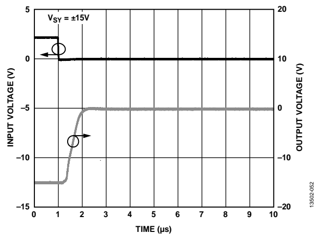
Figure 56. Negative Overload Recovery, A_V = -10 , V_{SV} = \pm 15V
