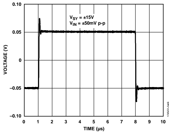
Figure 53. Small Signal Transient Response, V_{SV} = \pm 15V
