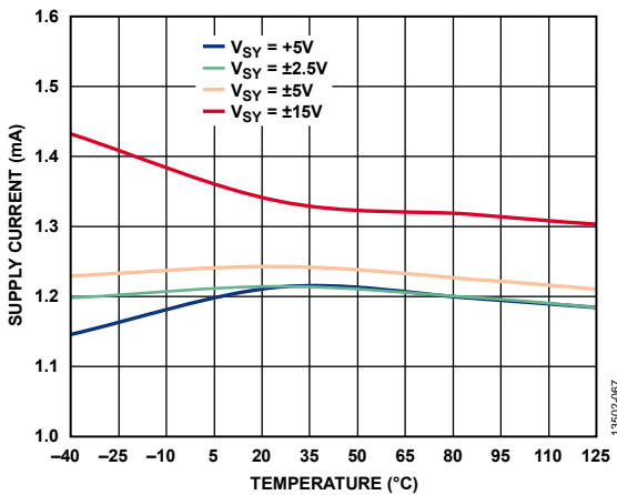
Figure 71. Supply Current ( I_{SV} ) vs. Temperature for Various Supply Voltages (ADA4622-2)
