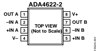
Figure 5. 8-Lead SOIC Pin Configuration, ADA4622-2
