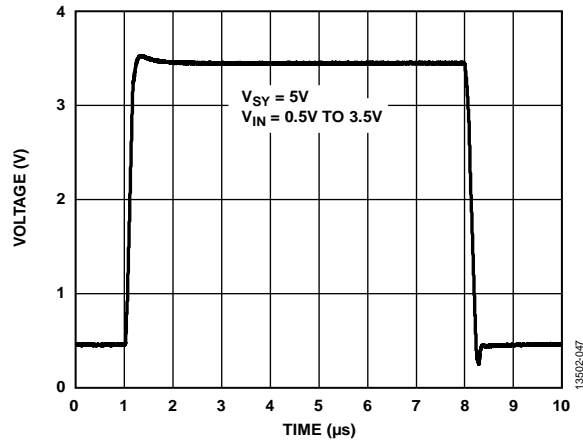
Figure 51. Large Signal Transient Response, V_{SV} = 5V
