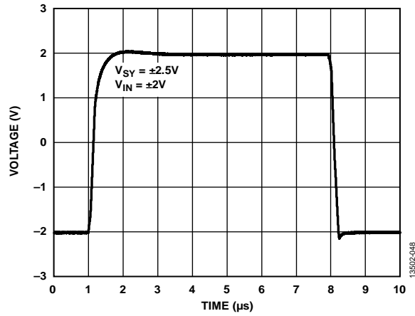
Figure 52. Large Signal Transient Response, V_{SV} = \pm 2.5V
