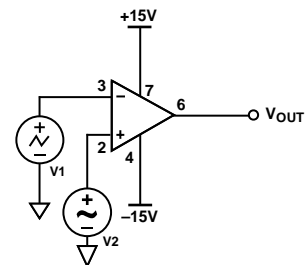
Figure 53. Pulse-Width Modulator
