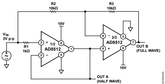
Figure 49. Half-Wave and Full-Wave Rectifiers
