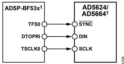
1 ADDITIONAL PINS OMITTED FOR CLARITY. 05943-038 Figure 36. Blackfin ADSP-BF53x Interface to AD5624/AD5664
