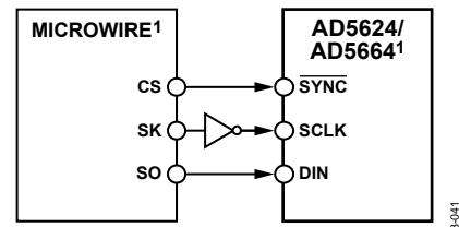
1 ADDITIONAL PINS OMITTED FOR CLARITY. 05943-041 Figure 39. MICROWIRE Interface to AD5624/AD5664
