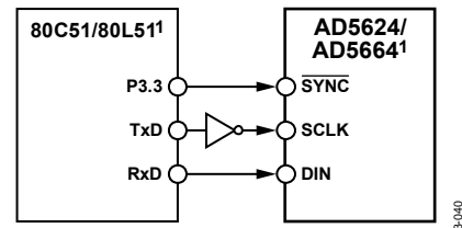
1 ADDITIONAL PINS OMITTED FOR CLARITY. 05943-040 Figure 38. 80C51/80L51 Interface to AD5624/AD5664
