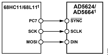
1 ADDITIONAL PINS OMITTED FOR CLARITY. 05943-039 Figure 37. 68HC11/68L11 Interface to AD5624/AD5664
