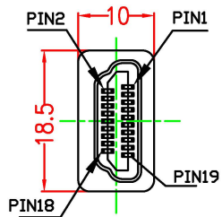
HDMI 19P MALE
