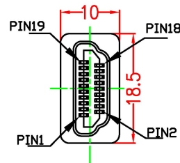
HDMI 19P MALE
